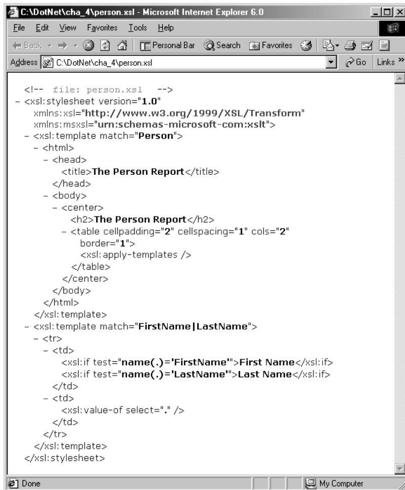
Figure 4.11 The XSLT rules for transforming Person.Xml
