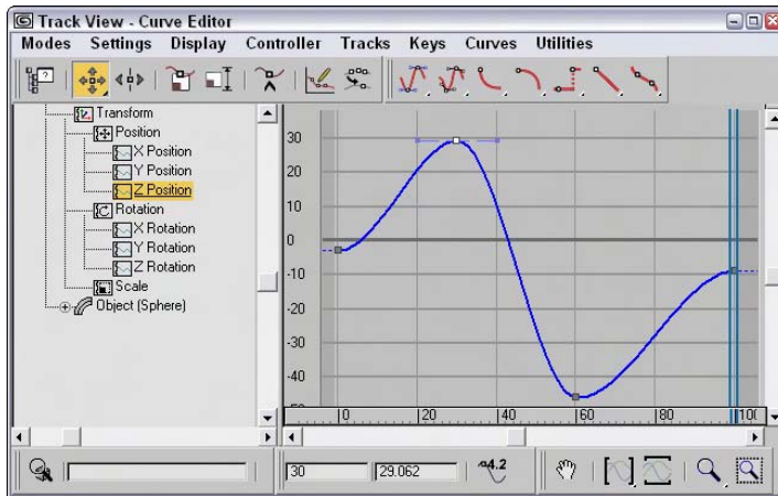
Figure 31-12: The Bézier controller produces smooth animation curves.
