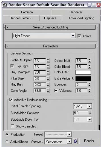
Figure 28-2: The Light Tracer Parameters rollout sets values for GI lighting.
