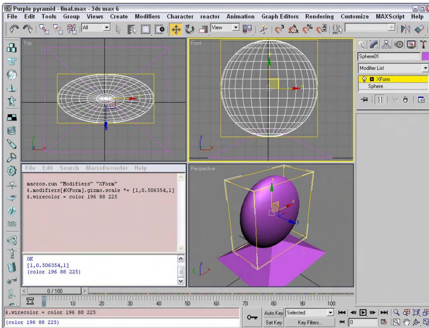
Figure 48-7: Running the new squash-and-turn-purple script
