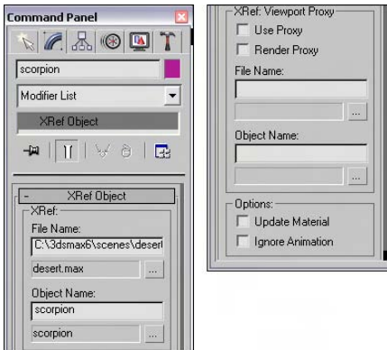
Figure 3-28: The XRef Object rollout in the Modify panel lets you choose which objects from which files to include as external references.
