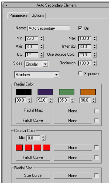
Figure 43-18: The Auto Secondary Element rollout sets the parameters for this effect.
