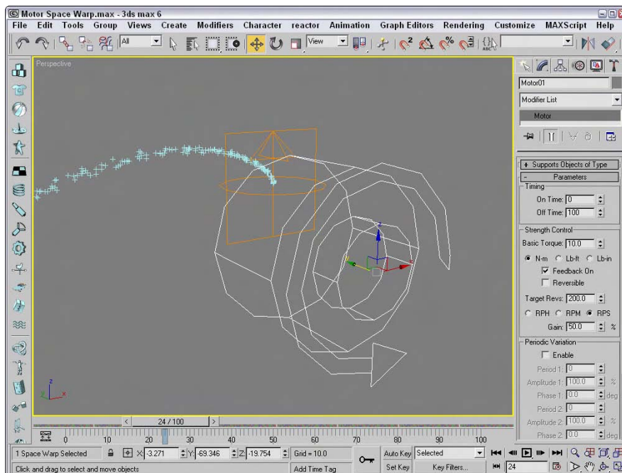
Figure 38-2: You can use the Motor Space Warp to apply a twisting force to particles and dynamic objects.
