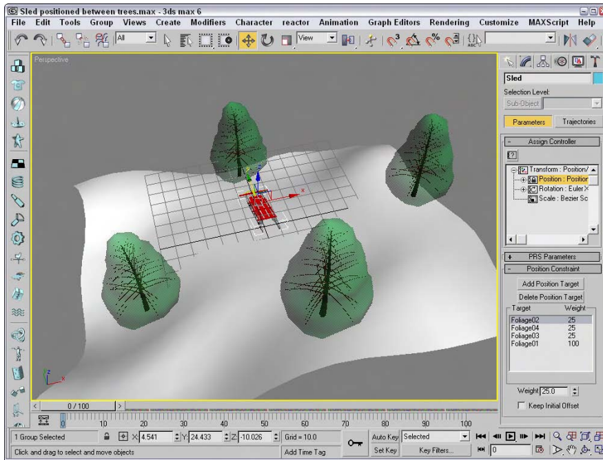
Figure 31-4: You can use the Position constraint to control the position of an object in relation to its targets.
