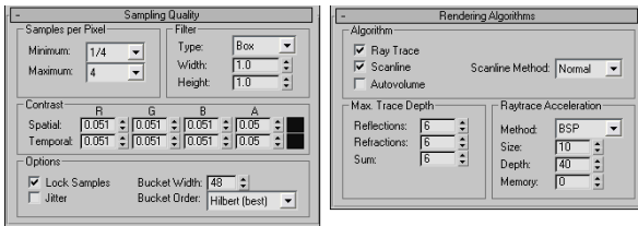
Figure 44-19: The Renderer panel includes several rollouts of settings for controlling the mental ray renderer.
