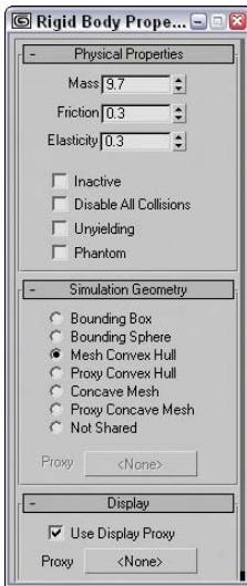
Figure 40-4: The Property Editor can set the physical properties for geometric objects included in the scene.
