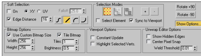
Figure 23-6: The Options pop-up interface includes many of the same features as the menus.
