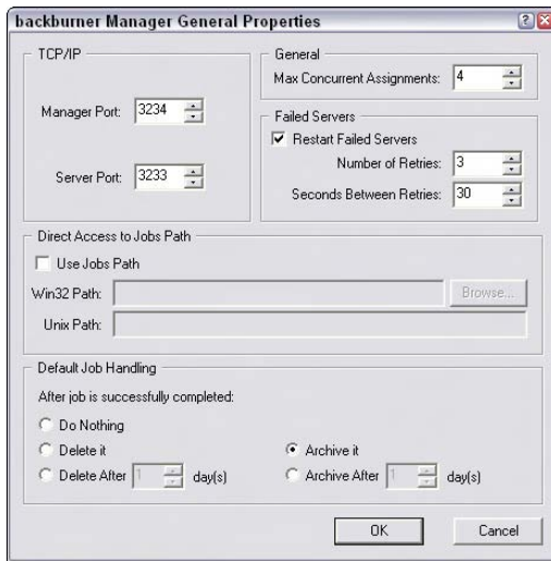
Figure 45-14: The backburner Manager General Properties dialog box
