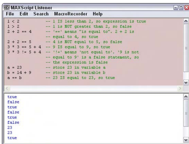
Figure 48-10: Using the MAXScript Listener to evaluate expressions
