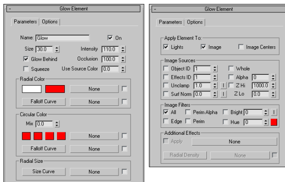
Figure 43-8: The Glow Element rollout lets you set the parameters for the Glow effect.
