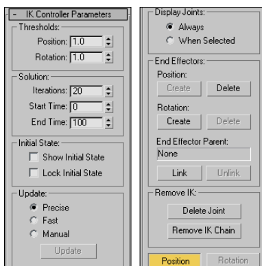
Figure 37-8: The IK Controller Parameters rollout sets the boundaries of the IK solution.
