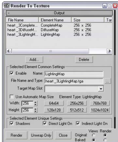
Figure 50-9: The Output rollout of the Render to Textures panel includes settings for specific objects.
