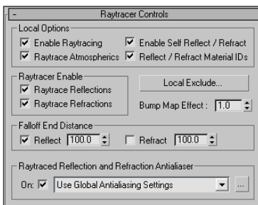
Figure 44-9: The Raytracer Controls rollout lets you set the raytracing options.
