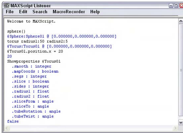
Figure 48-5: Use the MAXScript Listener window to query Max about an object's properties.
