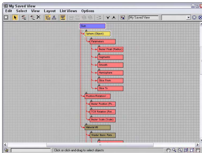
Figure 9-11: Without limiting nodes, the Schematic View window can get very busy.
