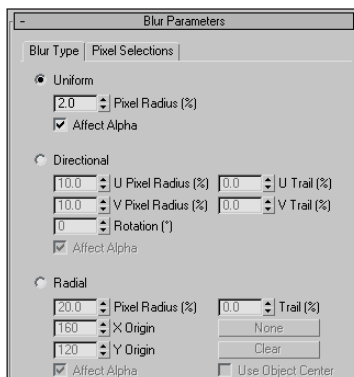
Figure 43-22: The Blur Parameters rollout lets you select a Uniform, Directional, or Radial blur type.
