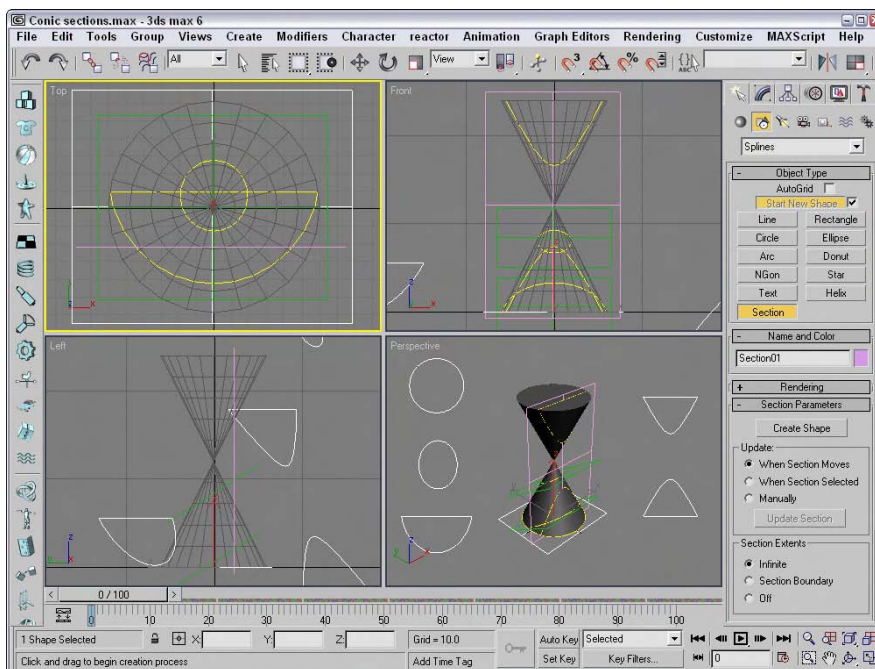
Figure 13-11: You can use the Section shape primitive to create the conic sections (circle, ellipse, parabola, hyperbola) from a set of 3D cones.
