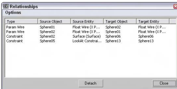
Figure 9-13: The List Views dialog box includes a list of nodes with relationships.
