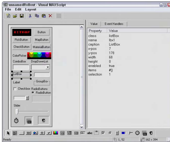
Figure 48-15: You can add control elements to the form in the Visual MAXScript window.
