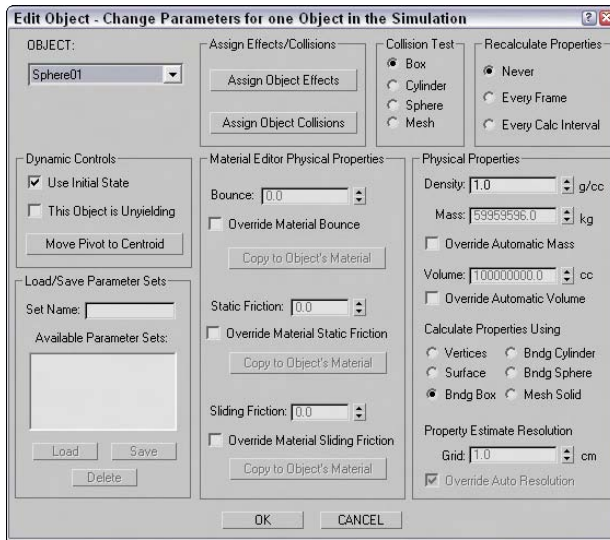
Figure 39-7: The Edit Object dialog box lets you assign simulation properties to an object.
