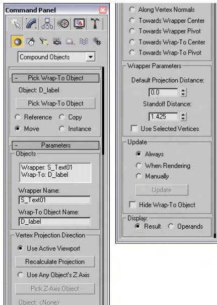
Figure 17-3: The Parameters rollout of the Conform object lets you define how the object is wrapped.
