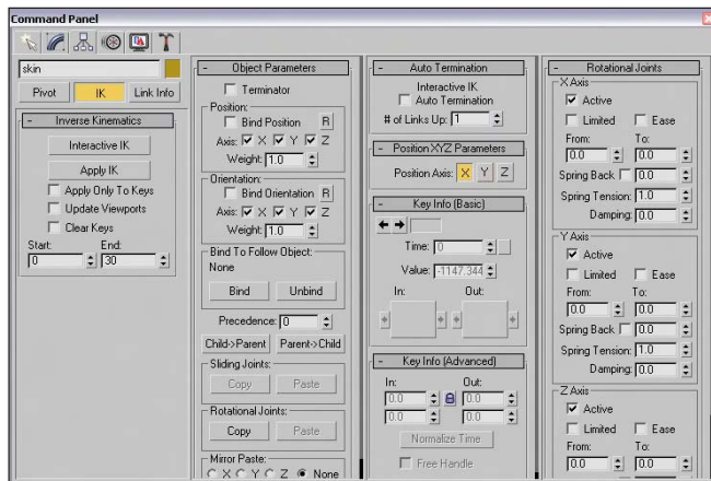
Figure 37-1: The IK rollouts let you control the binding of an IK system.
