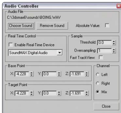
Figure 31-11: The Audio Controller dialog box lets you change values based on the amplitude of a sound file.
