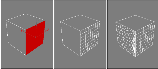
Figure 34-4: Avoid having to subdivide a single large face that shares an edge with many faces.
