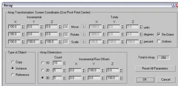
Figure 7-11: The Array dialog box defines the number of elements and transformation offsets in an array.
