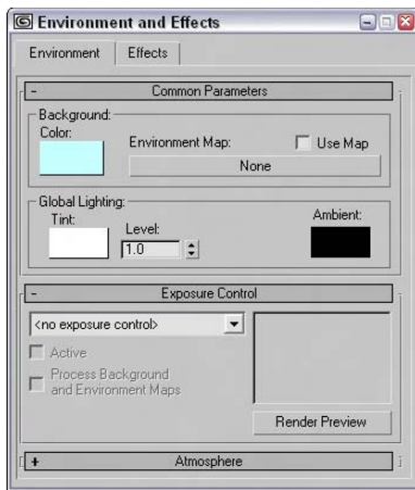
Figure 41-15: The Environment and Effects dialog box lets you select a background color or image, define global lighting, control exposure, and work with atmospheric effects.
