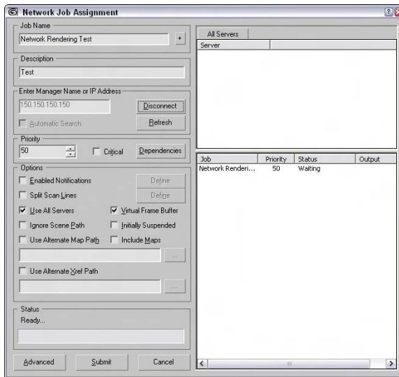
Figure 45-10: Using the Network Job Assignment dialog box to locate the manager to handle the rendering job
