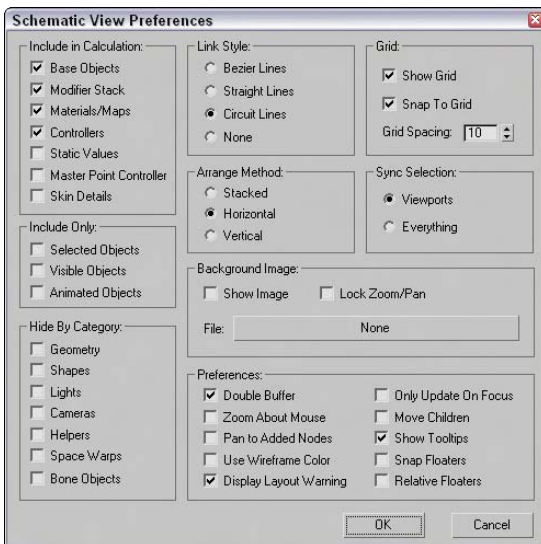
Figure 9-10: The Schematic View Preferences dialog box lets you customize many aspects of the Schematic View window.
