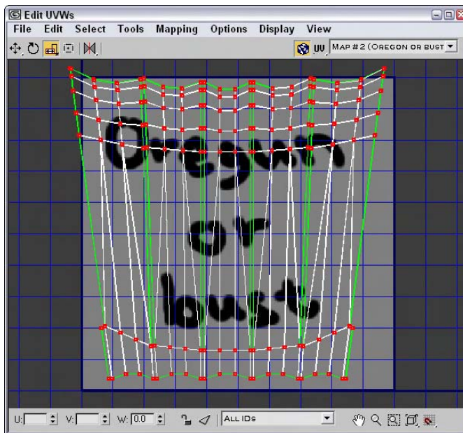
Figure 23-10: The Edit UVWs interface lets you transform the mapping coordinates by moving vertices.
