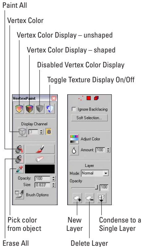
Figure 50-5: The Paintbox palette for the Vertex Paint modifier includes a wealth of features.
