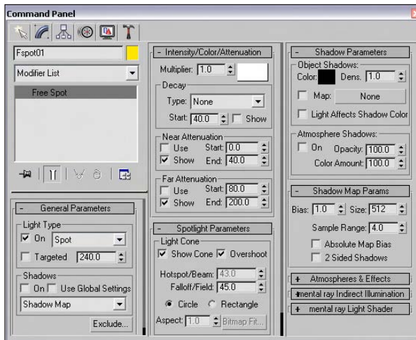
Figure 27-7: The various light rollouts control parameters and shadows.
