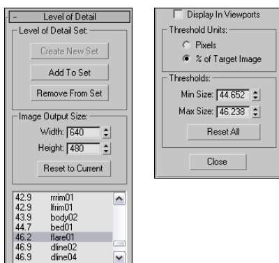
Figure 50-2: The Level of Detail utility (split into two parts) can specify how objects are viewed based on given thresholds.
