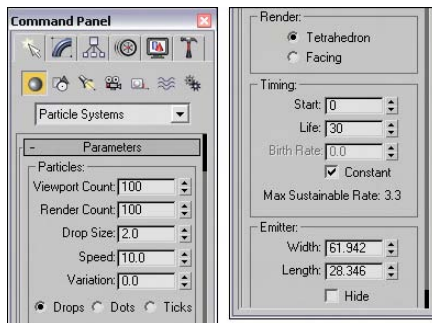
Figure 18-2: The Spray Parameters rollout holds the parameters for the Spray particle system.
