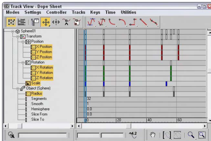
Figure 33-5: In the Dope Sheet, Position keys are red, Rotation keys are green, Scale keys are blue, and parameter keys are gray.
