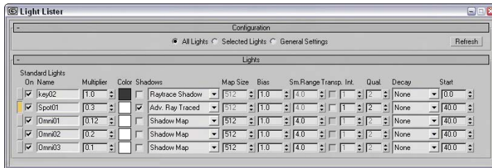
Figure 27-4: The Light Lister dialog box includes a comprehensive list of light settings in one place.
