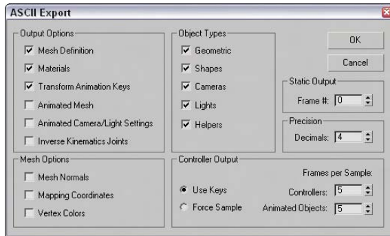
Figure 3-15: The ASCII Export dialog box exports the Max scene to a file that a text editor can read.
