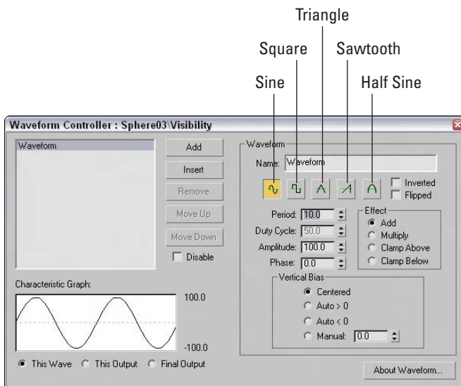
Figure 31-26: The Waveform Controller dialog box lets you produce sinusoidal motions.
