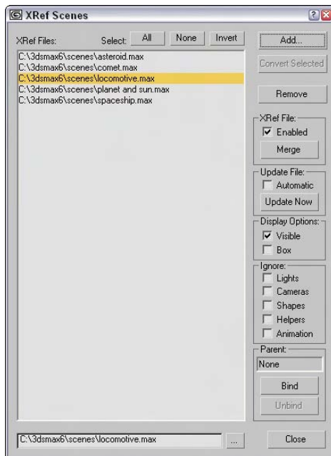
Figure 3-23: The XRef Scenes dialog box lets you specify which scenes to load as external references.
