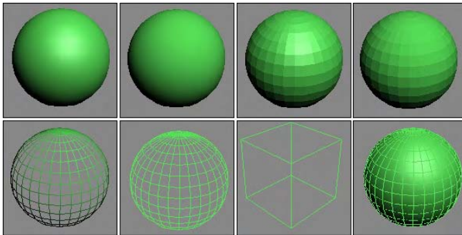
Figure 2-9: The viewport rendering methods from left to right are First Row: Smooth+Highlights, Smooth, Facets+Highlights, Facets. Second Row: Lit Wireframes, Wireframe, Bounding Box, and Edged Faces applied to Smooth+Highlights.
