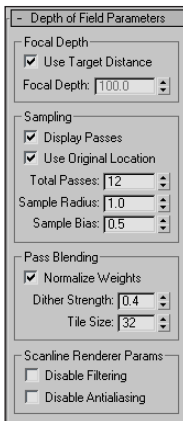
Figure 26-1: Use the Depth of Field Parameters rollout to set the number of passes.
