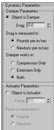
Figure 39-3: The Dynamics Parameters section of the Damper Parameters rollout defines the physical characteristics of the damper object.
