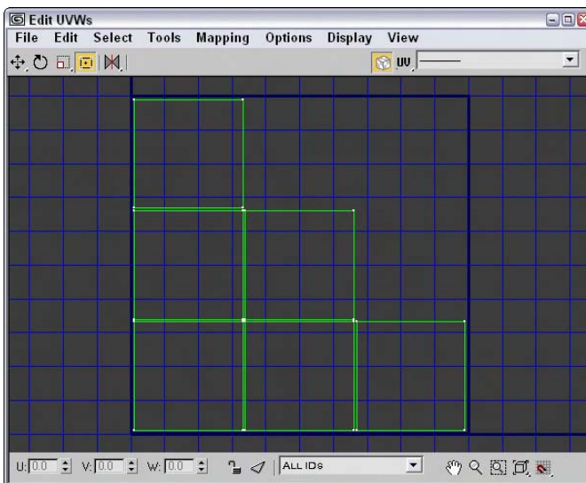
Figure 23-5: The Edit UVWs interface lets you control how different planar maps line up with the model.
