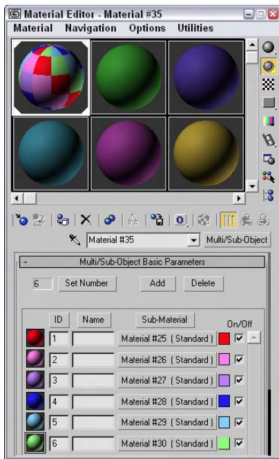
Figure 21-3: The Multi/Sub-Object material defines materials according to material IDs.
