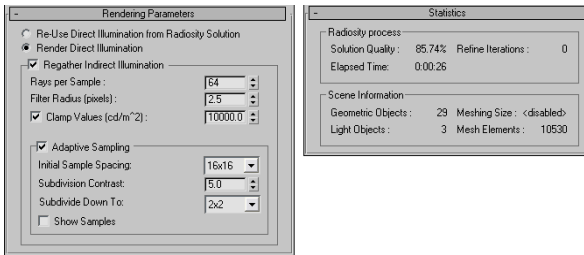
Figure 29-6: The Rendering Parameters and Statistics rollouts offer rendering options and statistics for radiosity solutions.
