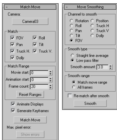
Figure 25-9: The Match Move and Move Smoothing rollouts let you select a camera to match to the tracking data and smooth the camera’s motion.
