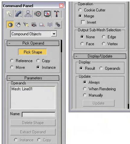
Figure 17-5: Use the Parameters rollout for the ShapeMerge compound object to cut or merge a shape.
